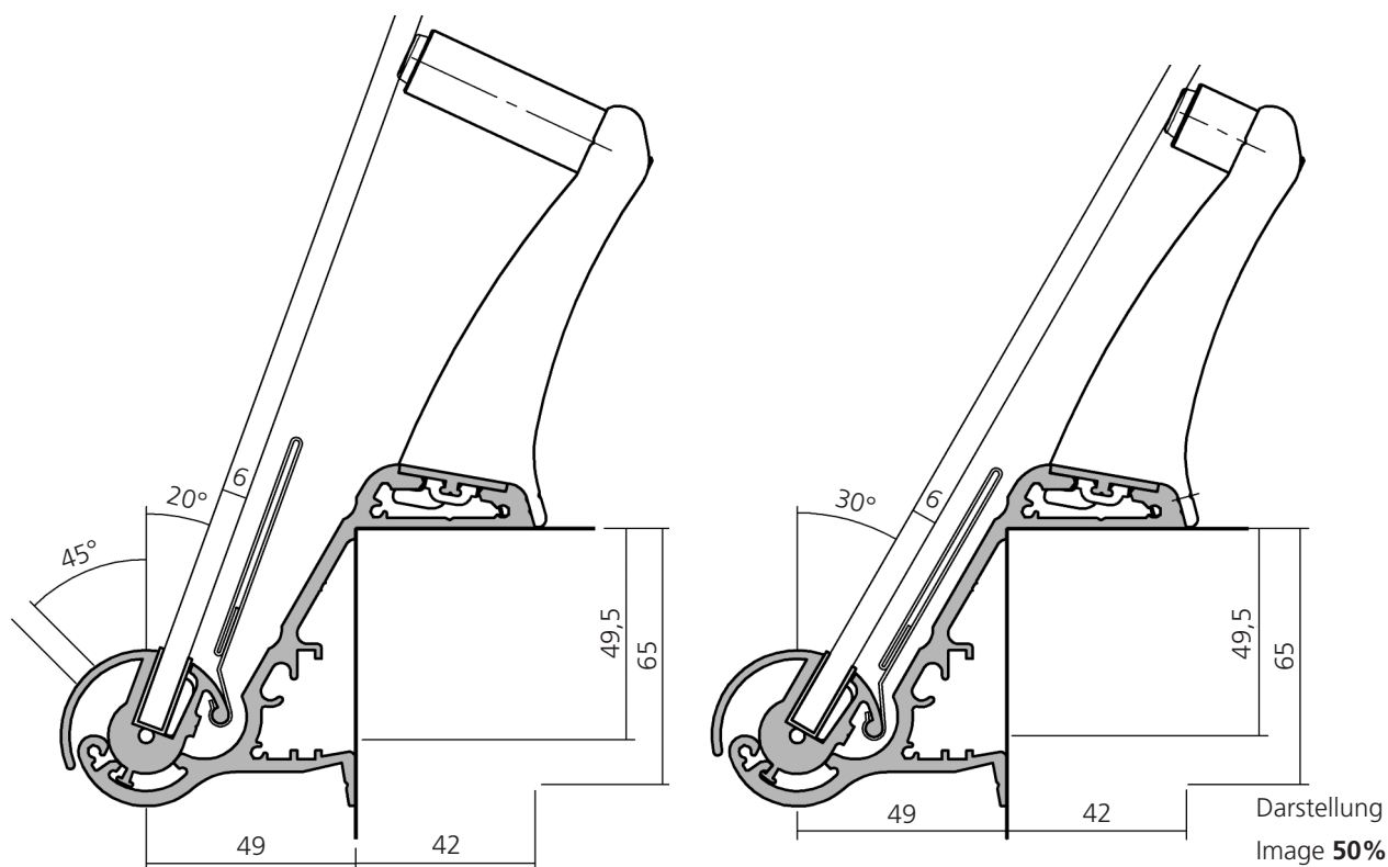
Anschlagprofil, Aluminium Stop profile
