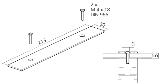
Deckleiste – Mitte, Aluminium Covering profile – centre
