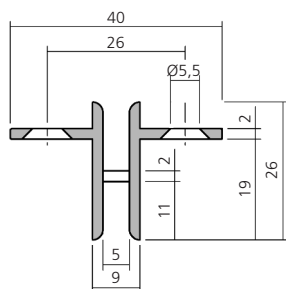
Rasterschiene, Aluminium Slotted rail
