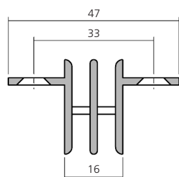
Rasterschiene, Aluminium Slotted rail
